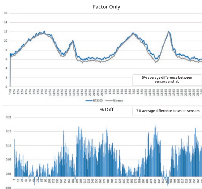
Figure 1. Demonstration of effectiveness of Factor vs Offset when comparing NT3100sc and Nitratax.
