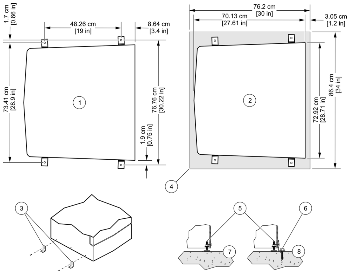
Figure 2 Installation of anchor bracket mounts
